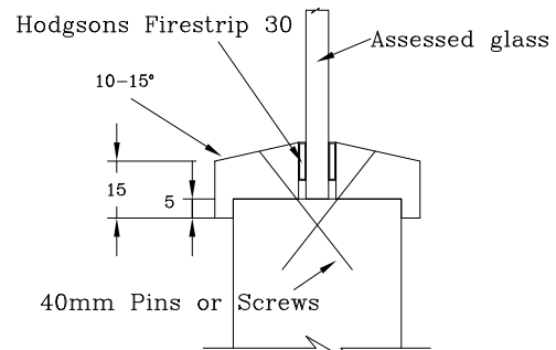
Hodgsons Sealants Ltd Firestrip 30
