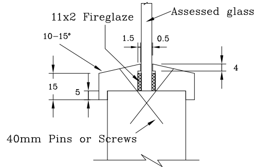
Sealmaster Ltd Fireglaze
