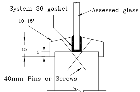
Lorient Polyproducts Ltd System 36
