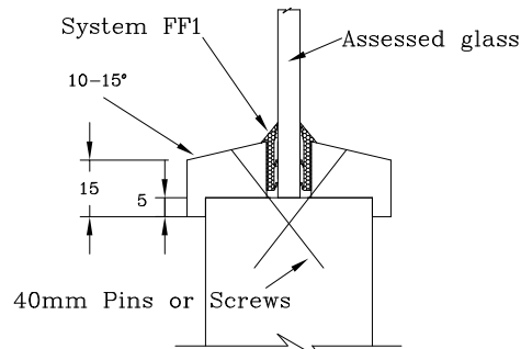
Lorient Polyproducts Ltd System FF1
