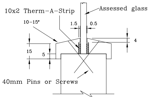
Intumescent Seals Ltd Therm-A-Strip
